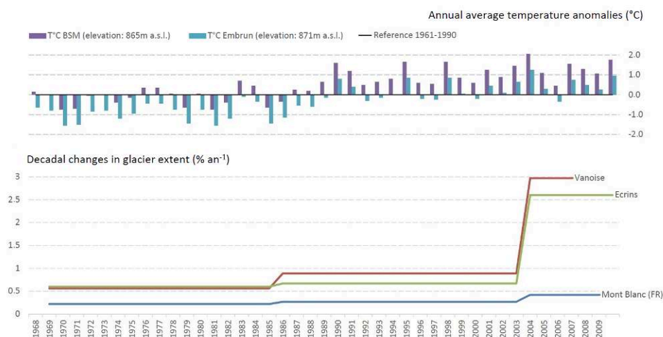
Figure 2: (A) Annual average temperature anomalies in Bourg-Saint-Maurice and Embrun over the period 1967-2010 compared to the 1961-1990 normal (see Fig. 1). (B) Estimation of decadal changes in glacial extent in the main massifs of the French Alps for different periods from 1967/71 to 2006/09, expressed in % per year (Gardent et al. , 2014)
